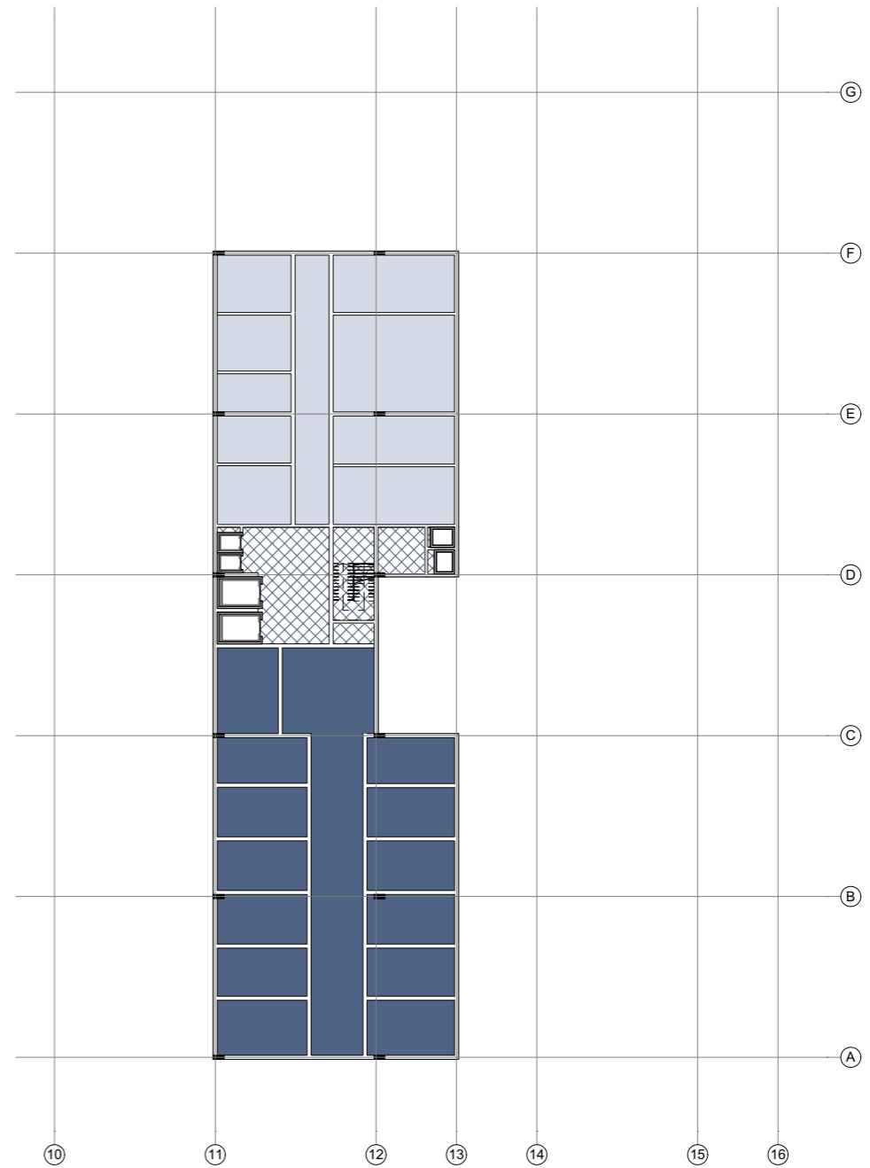
5. NADSTROPJE
