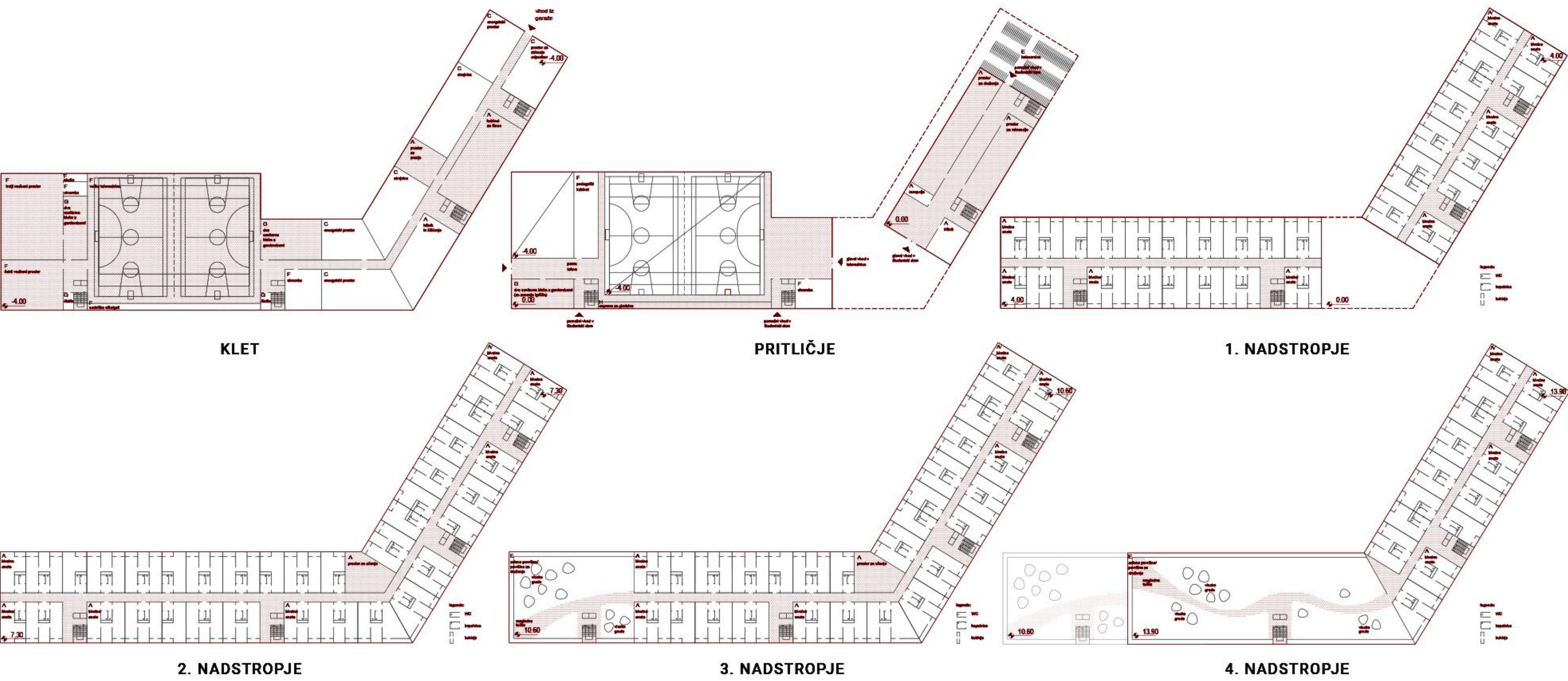
PROGRAMSKA SHEMA ŠDL IN TELOVADNICA M 1: 500
