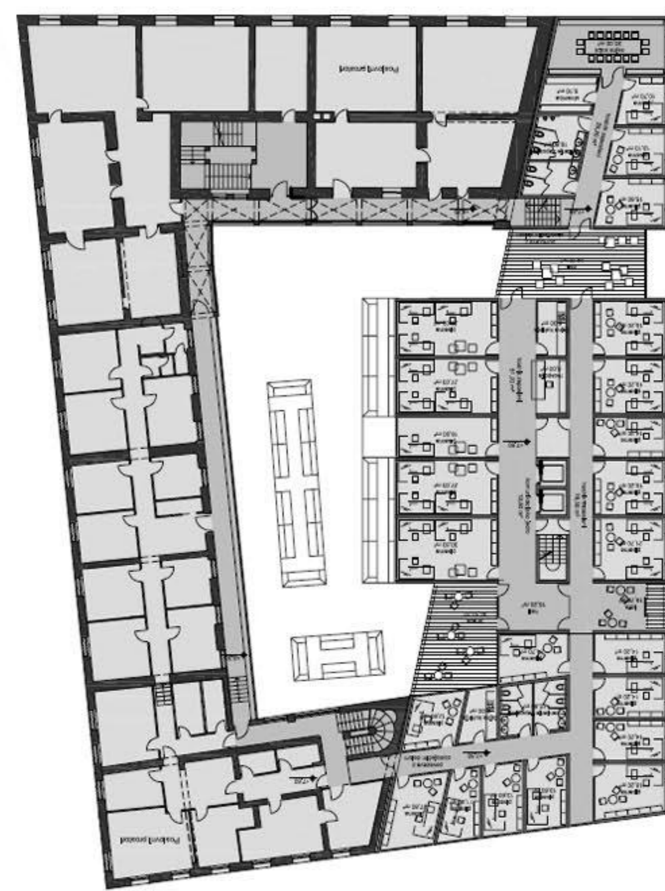
ETAGE 1, NADSTROPJA MAHROVE HISE 1:200
