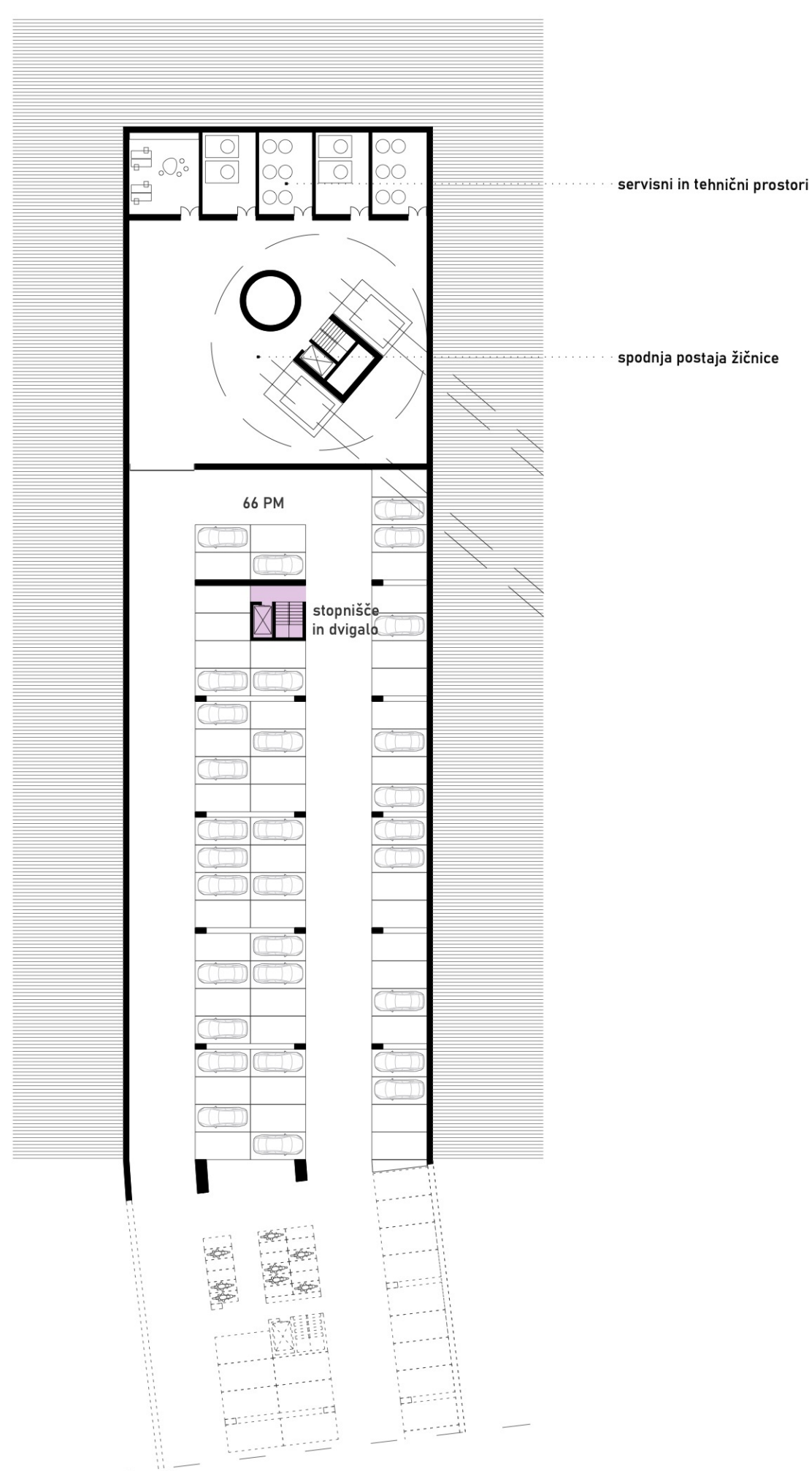
TLORIS KLETI -3.9m (faza 2) M 1:500
